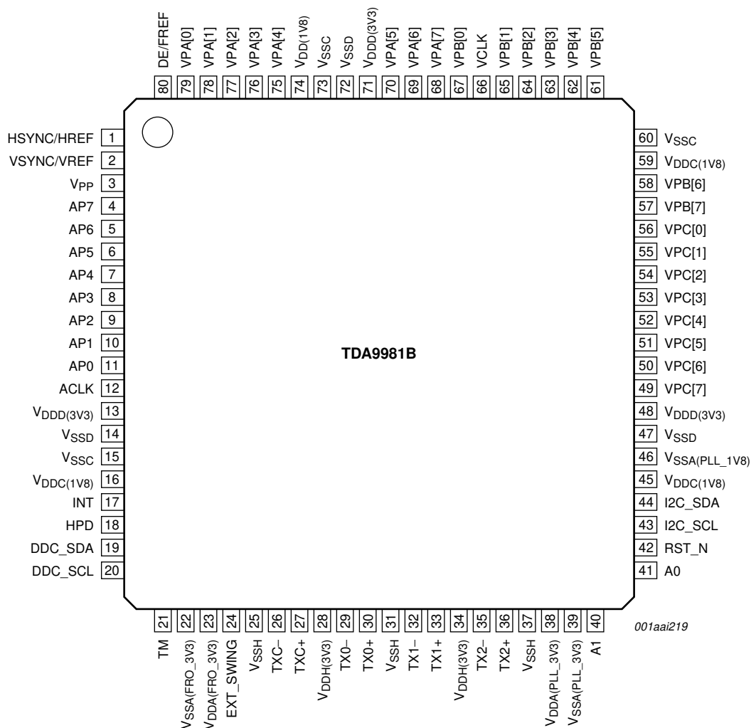
Fig 2. Pin configuration
